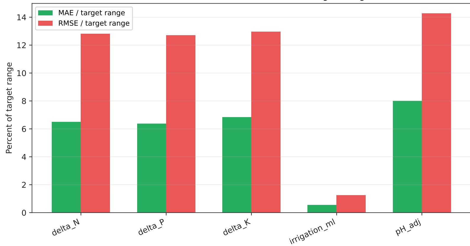
Normalized Error Relative to Test-Set Target Range
